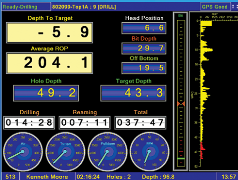
Operator Display
